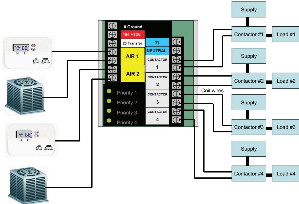
Load Shed Module Connections
